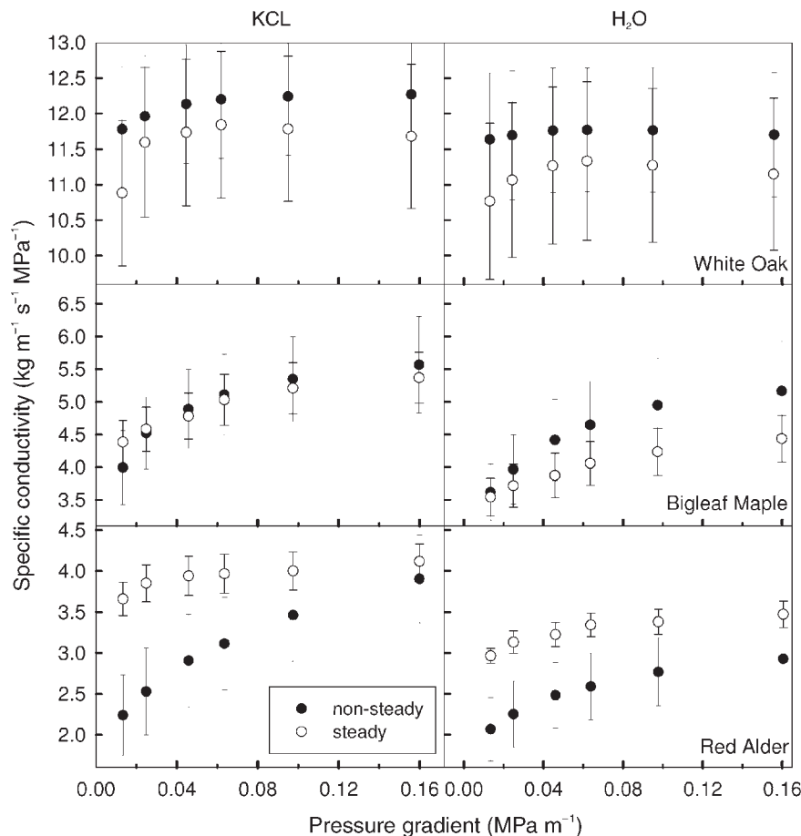
Figure 6. Specific conductivities of angiosperm stem xylem in relation to steady and non-steady pressure gradients using either deionized water ( \text{H}_2\text{O} ) or 25 mmol KCl as the perfusion fluid (mean \pm SE, n = 4 ).
